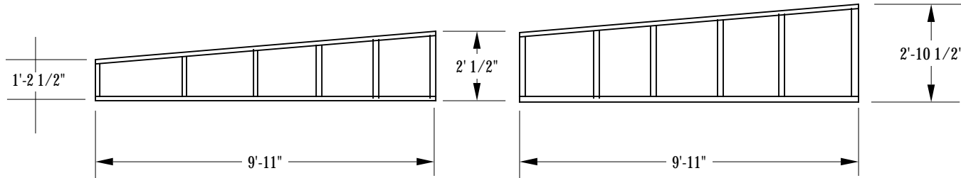
RAKE FRAMES - BUILD FIVE (5) EACH - UNITS BOLT TOGETHER
