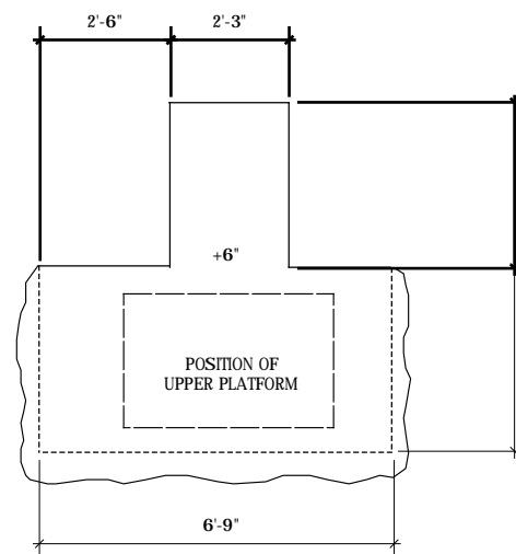
BASE PLATFORM TOP VIEW
