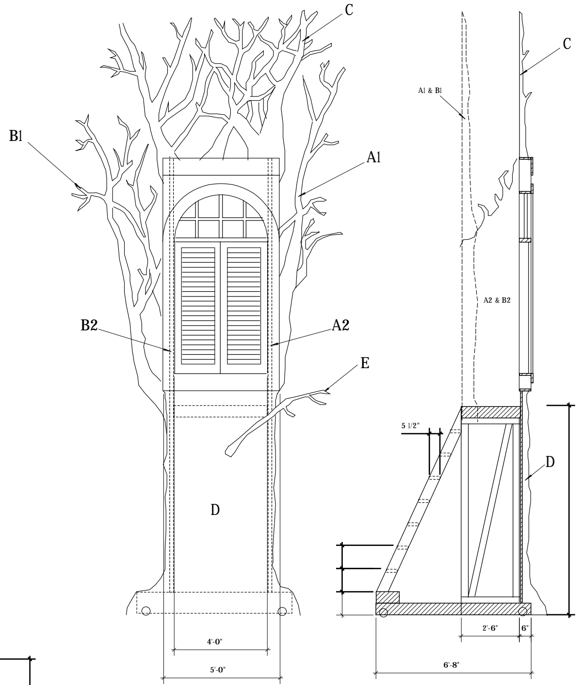
FRONT ELEVATION
