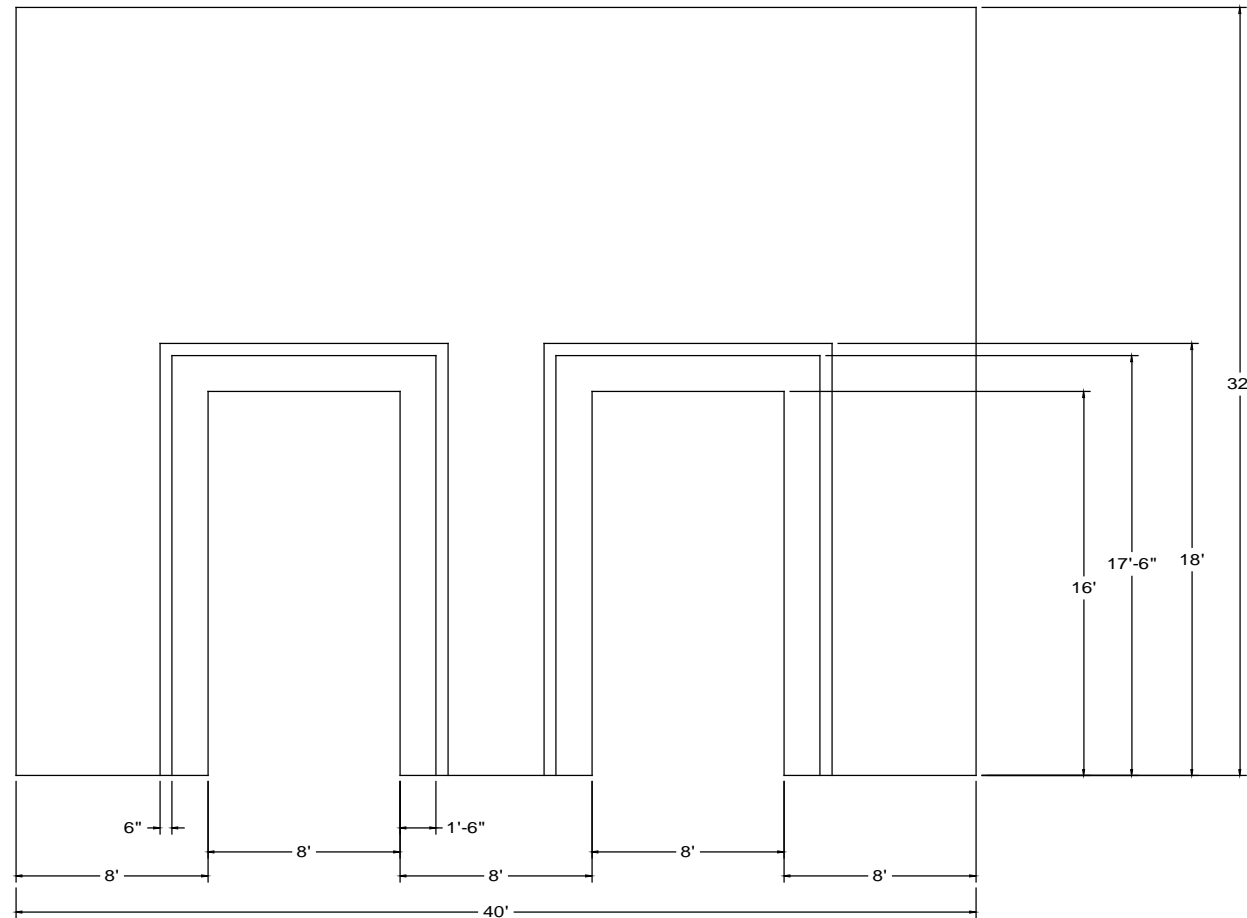
BIG WALL FRONT ELEVATION
