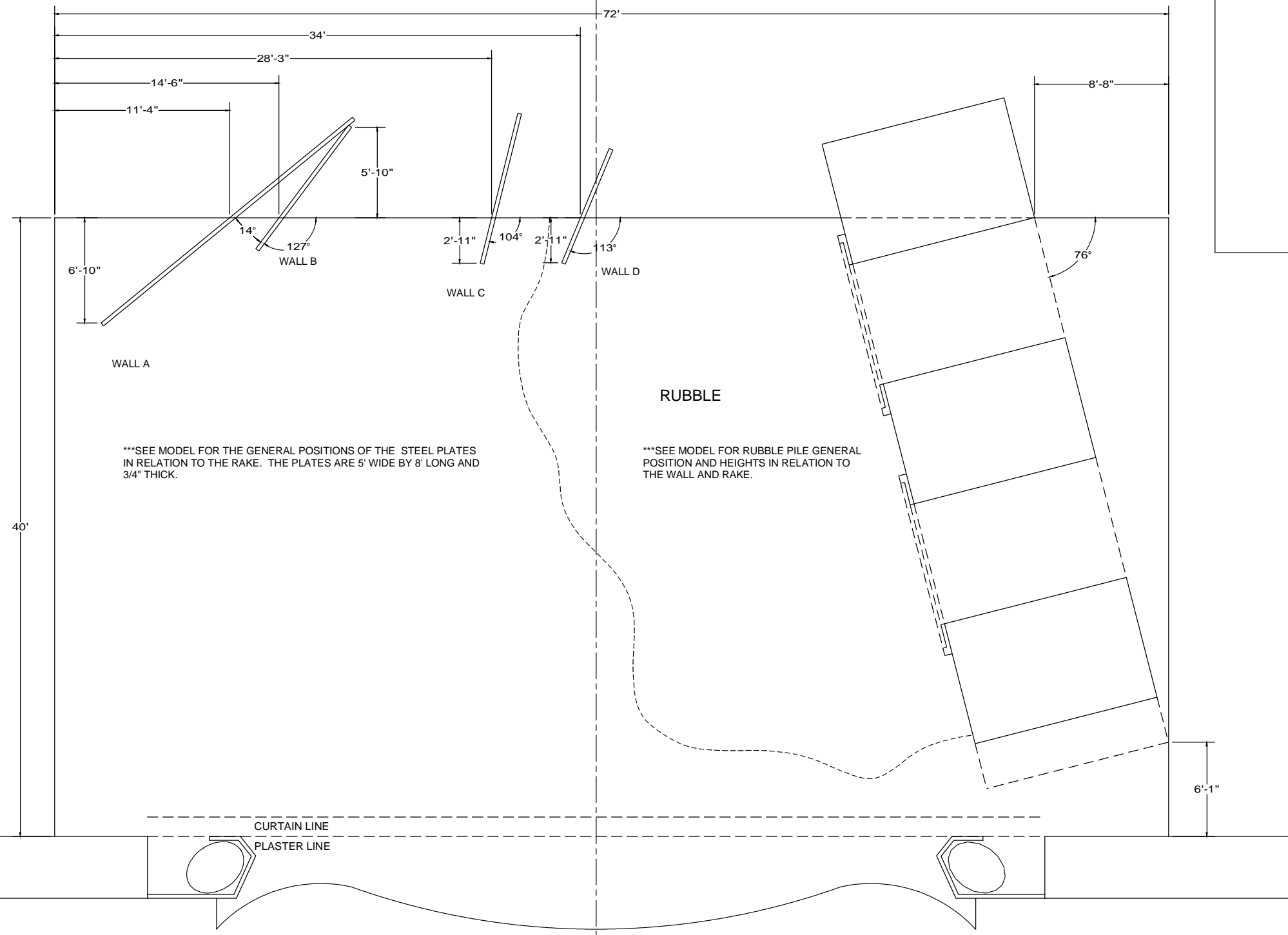
PLAN VIEW
